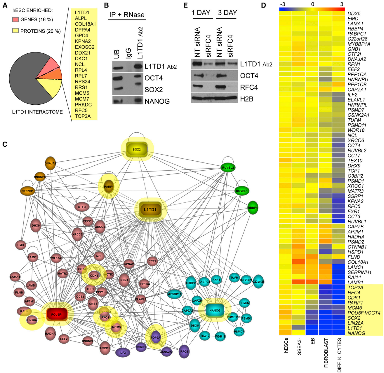
Figure 4. L1TD1 Connects Uncharacterized Factors to Core Pluripotency Regulation
