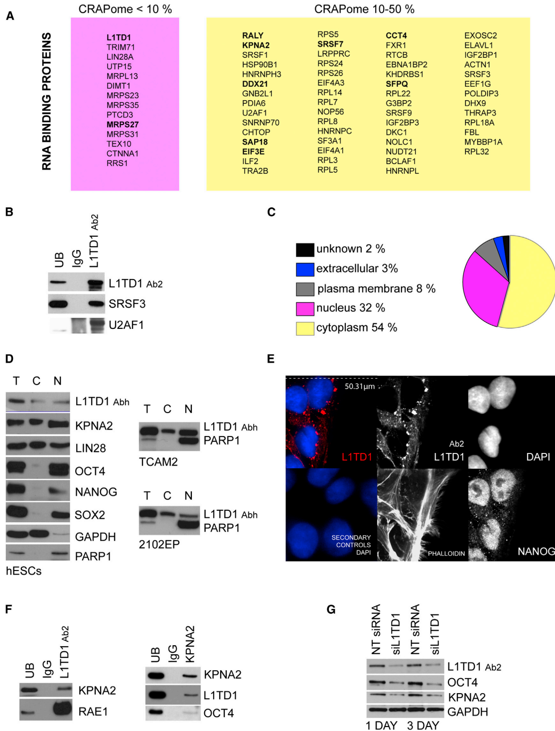
Figure 2. The L1TD1 Interactome Uncovers the Importance of RBPs and the Potential Role of L1TD1 in Nuclear Pore Traffic
